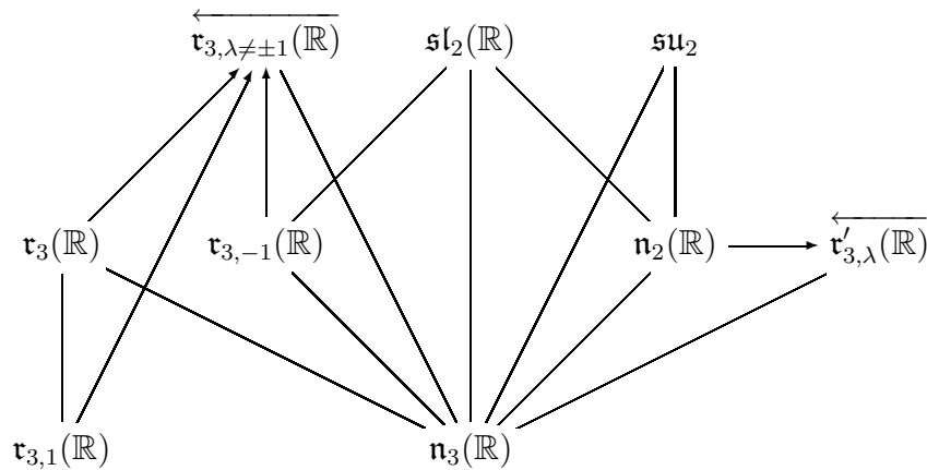
Fig.2 Contractions and deformations of the three-dimensional real Lie algebras
