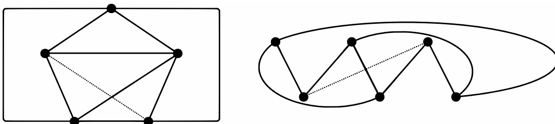
Figure 1.15. The graphs K_5 and K_{3,3} are not planar.
