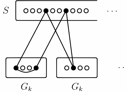
Figure 1.7. A possible \mathcal{C}_5 in G_{k+1} .
