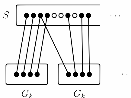
Figure 1.6. The construction of the graph G_{k+1} .
