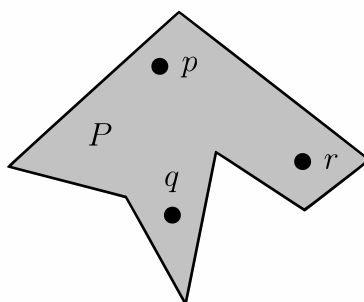
Figure 1.8. The p is visible from q and r . But q and r are not visible to each other.
