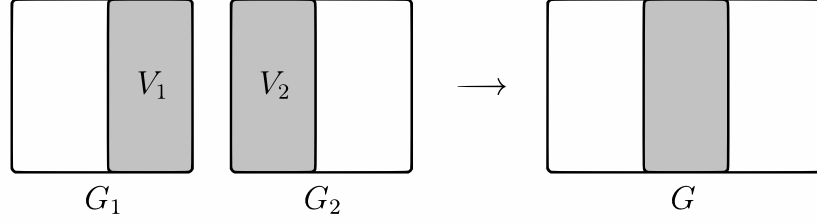
Figure 1.12. Pasting along a clique.
