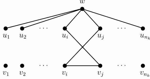
Figure 1.3. Mycielski's construction of G_{k+1} .
