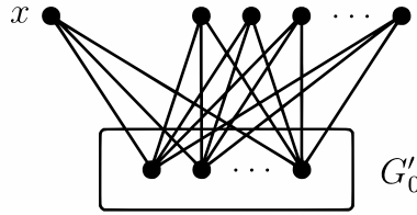
Figure 3.1. The graph G' .
