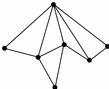
Figure 1.10. Triangulation of a 7-gon.
