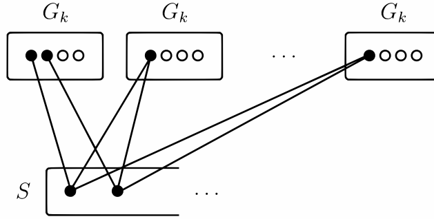
Figure 1.2. Zykov's construction of G_{k+1} .
