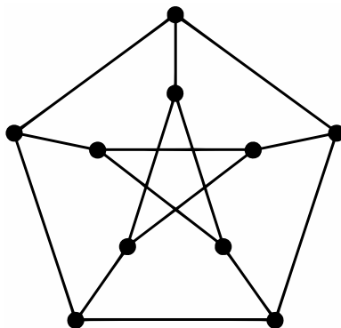
Figure 1.16. The Petersen graph.
