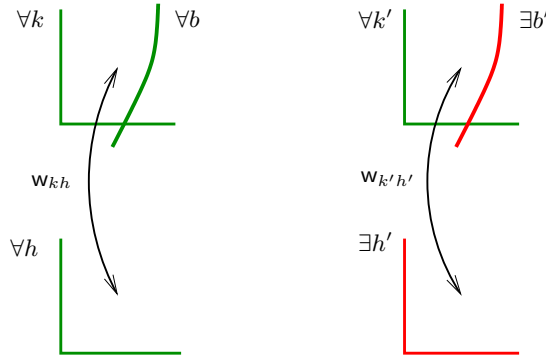
Fig. 4. Illustration for \text{SPR}_B and \text{SPR}_{IOb} .
