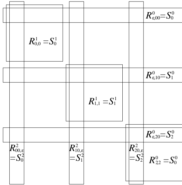
Figure 1. The family \mathcal{R} = \mathcal{R}(3, 2) . Equal coordinates are slightly perturbed for clarity.
