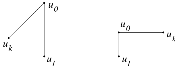
Figure 3. Find the right position for u_0 .
