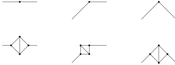
Figure 1. Replacing v by \Theta .
