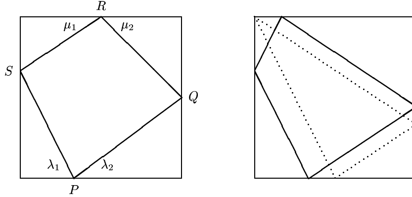
Figure 10: An extremal quadrangle
