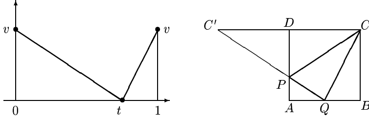
Figure 14: Triangle with equal slopes at P
