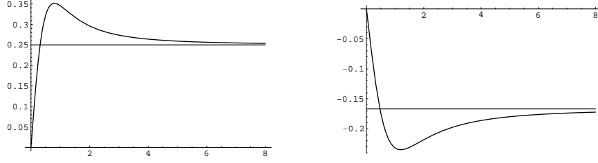
Figure 2: h(x) for a = 0.8 and a = 1.2
