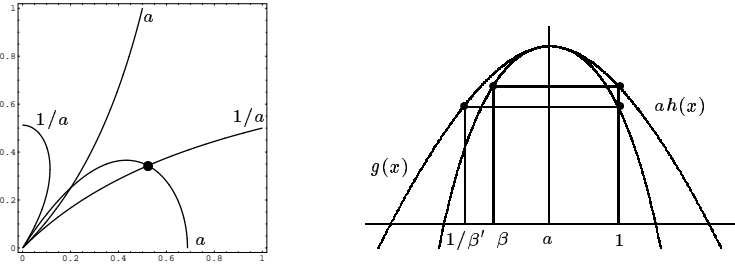
Figure 13: Superposing H(a) and H(1/a) for a = 0.8
