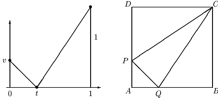
Figure 11: The triangle case
