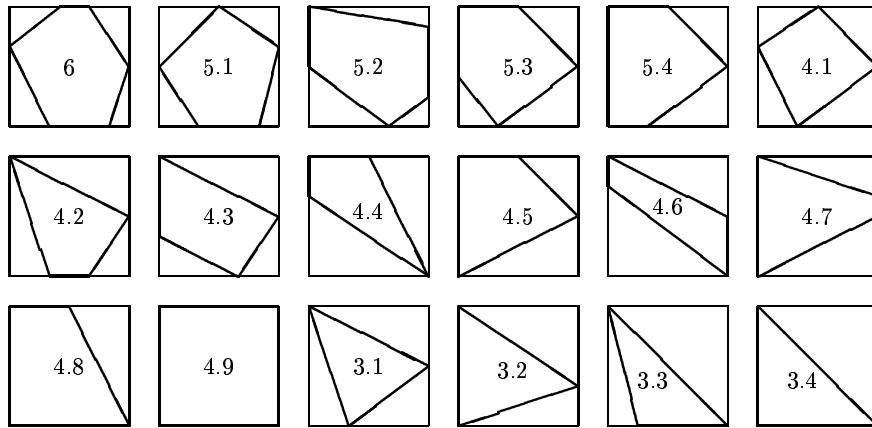
Figure 5: Classification of extremal polygons
