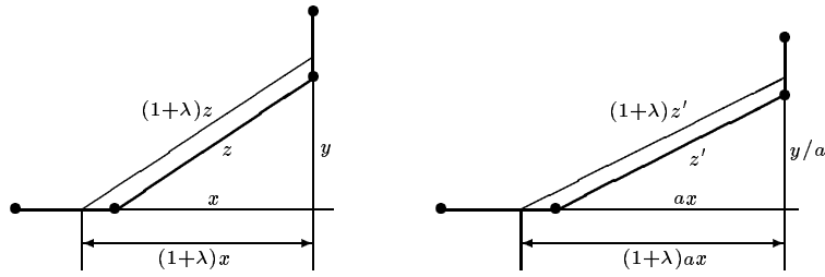
Figure 4: Vertices on two adjacent sides
