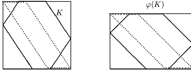
Figure 7: The hexagonal case
