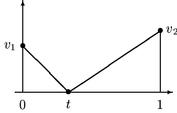
Figure 8: Vertex in an internal point
