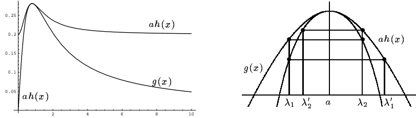
Figure 9: g(x) and ah(x) for a = 0.8
