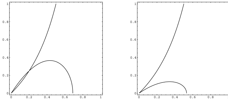
Figure 12: The set H(a) for a = 0.8 and a = 1.2
