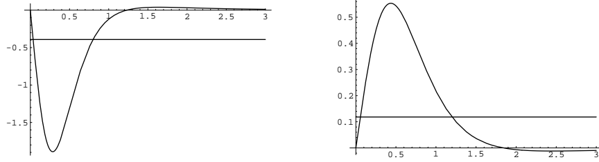
Figure 15: h''(x) for a = 0.8 and a = 1.2
