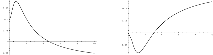
Figure 3: g(x) for a = 0.8 and a = 1.2
