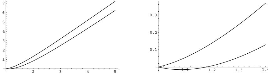
Figure 16: Maximal and minimal changes in the perimeter
