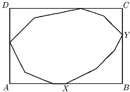
Figure 1: An inscribed convex polygon
