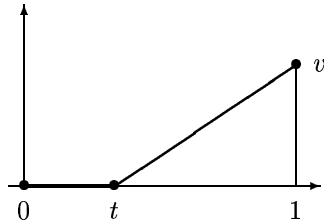
Figure 6: Two vertices on a single side
